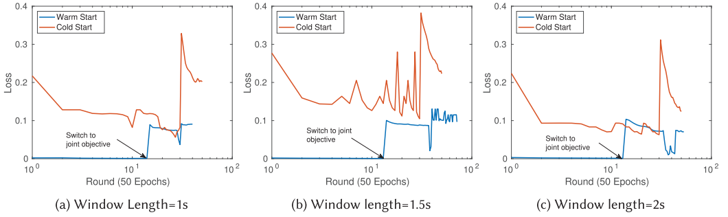
Fig. 10. Training loss landscapes of MSC-RNN joint optimization with ( warm start ) and without ( cold start ) pre-training of the two tiers ( H=64 ).
