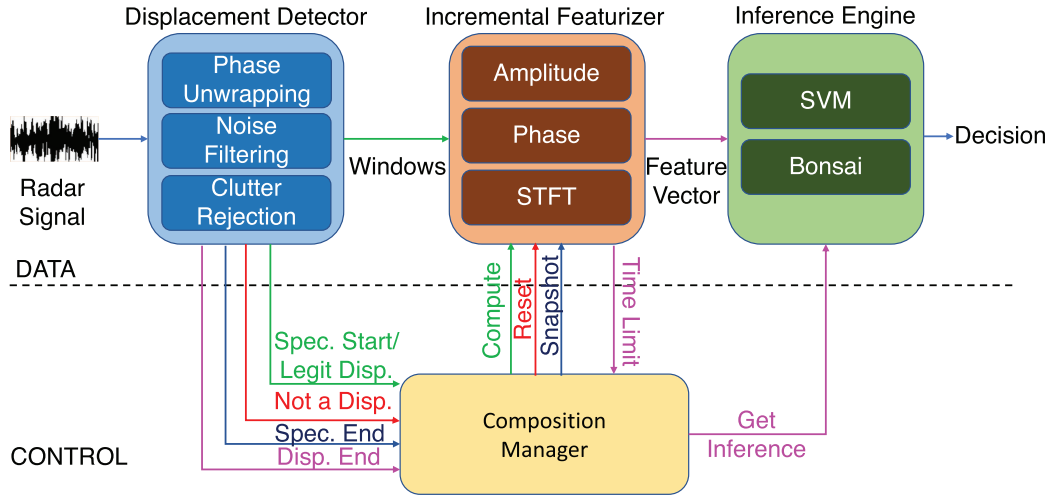
Fig. 3. SVM classifier data and control planes; control signal-response pairs are color coded.
