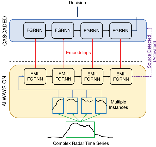
Fig. 5. MSC-RNN architecture – The lower EMI-FastGRNN runs continuously, while the higher FastGRNN is invoked only for legitimate displacements.
