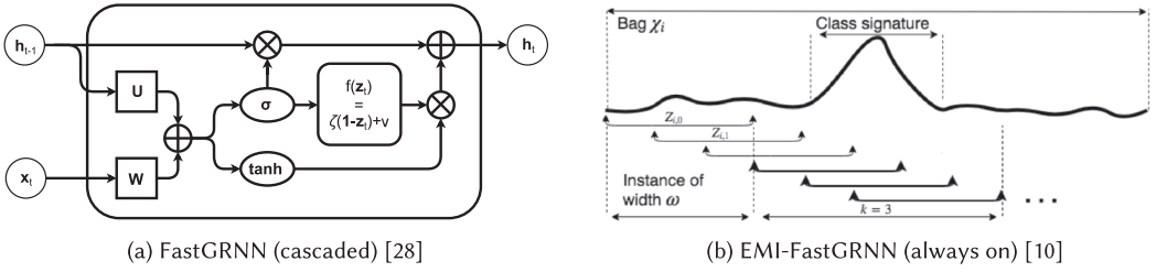
Fig. 4. FastGRNN & EMI-FastGRNN (©Aditya Kusupati et al. [28], ©Don Dennis et al. [10]).
