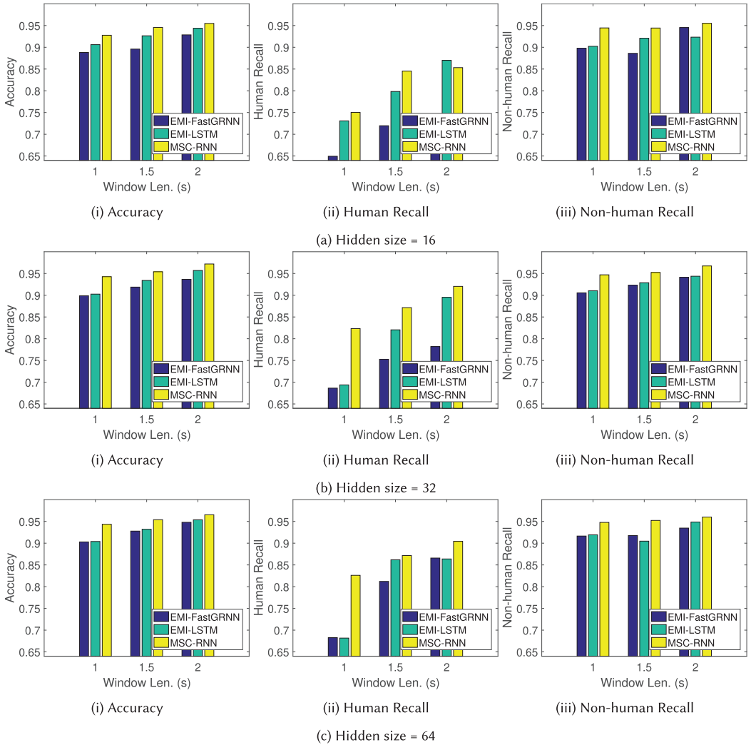
Fig. 11. Sensing performance comparison of MSC-RNN with EMI-FastGRNN and EMI-LSTM.
