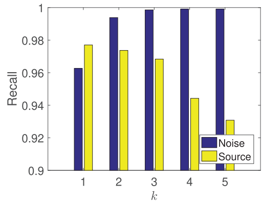
(b) Impact of k on EMI Recalls
