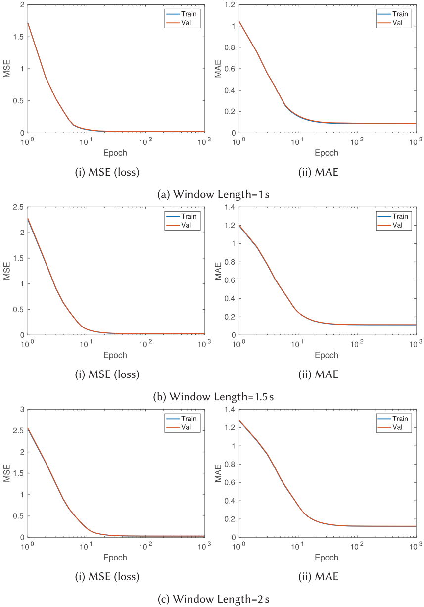
Fig. 12. Evolution of training and validation loss (MSE) and MAE with a FastGRNN setup to approximate the top 16 cross-domain handcrafted features for radar classification, purely from time domain input. N.B. : The training and validation MSEs and MAEs almost overlap in each training, indicating no over-/underfitting.
