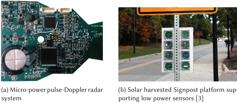
Fig. 1. The micro-power pulse-Doppler radar (PDR) device can be independently deployed or interfaced with existing multi-sensor smart city platforms such as Signpost (©Joshua Adkins et al. [3]).
